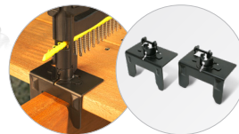
PDECKNC-RC (sold separately) The decking nose clip positions the screw on the deck board and positions it over the joist for an easy, uniform installation from a standing position.
