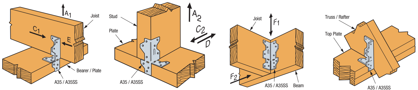
A35/A35SS Joist-to-Bearer/Plate
