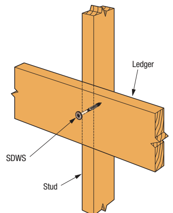
SDWS Ledger-to-Stud Connection
