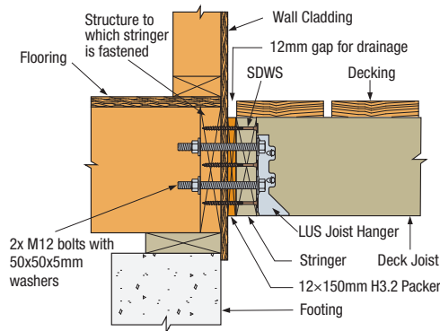
SDWS Stringer-to-House for Deck Connection
