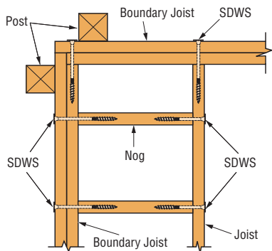
SDWS Deck Joist Fixing - Plan View
