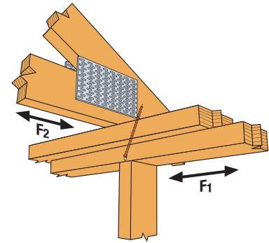
Typical single SDWC installation
