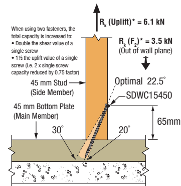
Stud-to-bottom plate condition over concrete/masonry foundation (This application requires SDWC15450)
