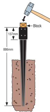
Typical Installation
