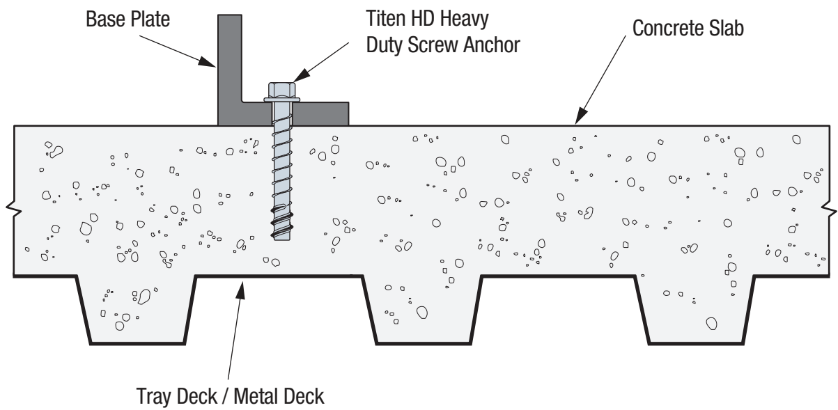
SIMPSON Strong-Tie® Titen HD Fastening on Tray Deck / Metal Deck
