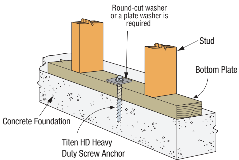
SIMPSON Strong-Tie® Titen HD Bottom Plate Fixing
