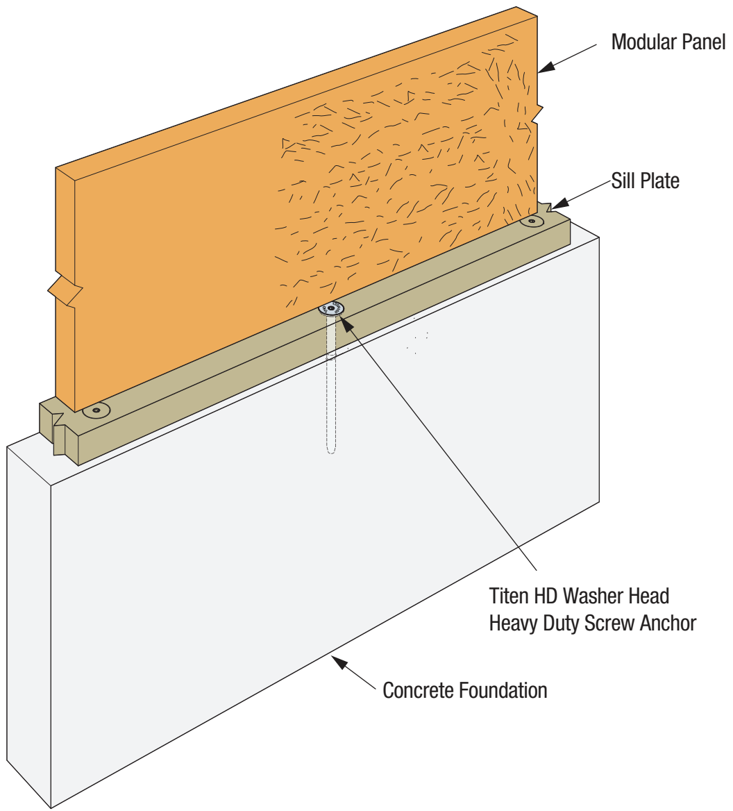
SIMPSON Strong-Tie® Titen HD Washer Head Sill Plate Modular Floor Installation
