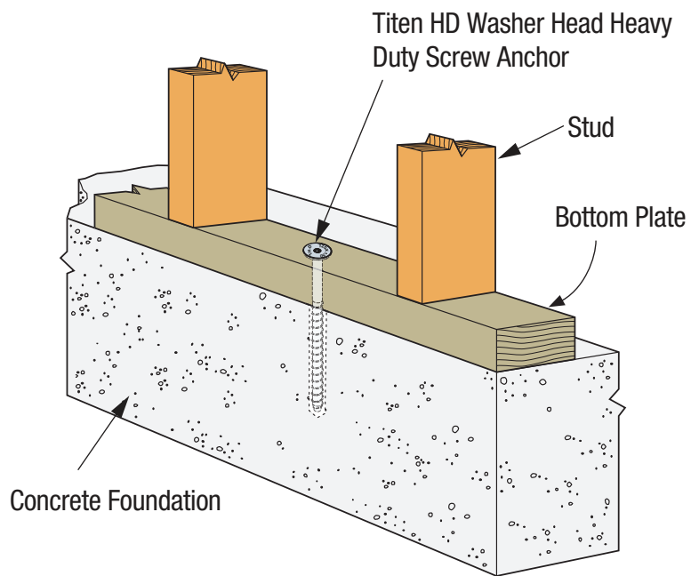
SIMPSON Strong-Tie® Titen HD Washer Head Bottom Plate Fixing
