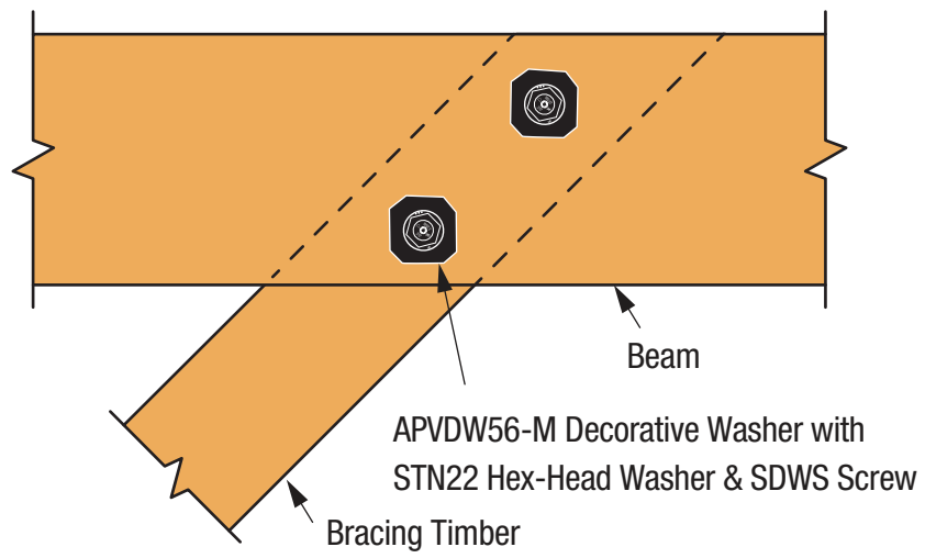
SIMPSON Strong-Tie® STN22 & SDWS Timber Brace Connection with Beam
