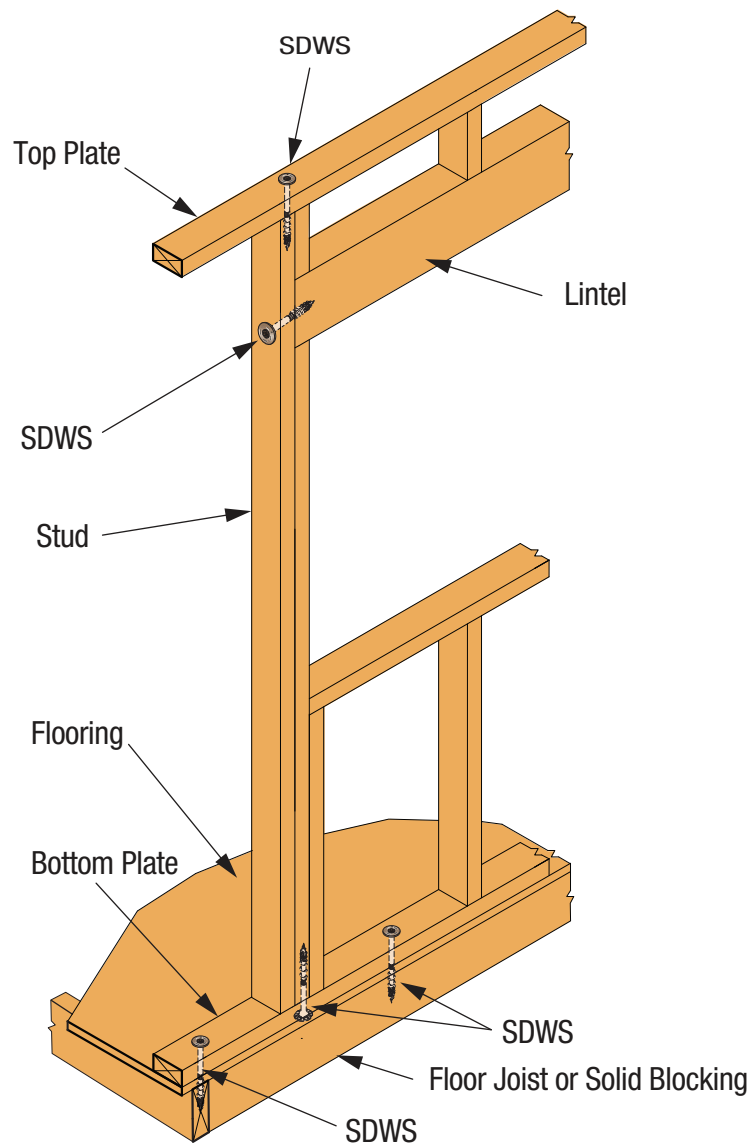
SIMPSON Strong-Tie® SDWS Stud-to-Top/Bottom Plate Stud-to-Lintel Bottom Plate-to-Joist Connection
