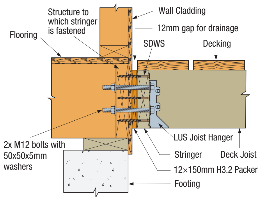
SIMPSON Strong-Tie® SDWS Stringer-to-House for Deck Connection
