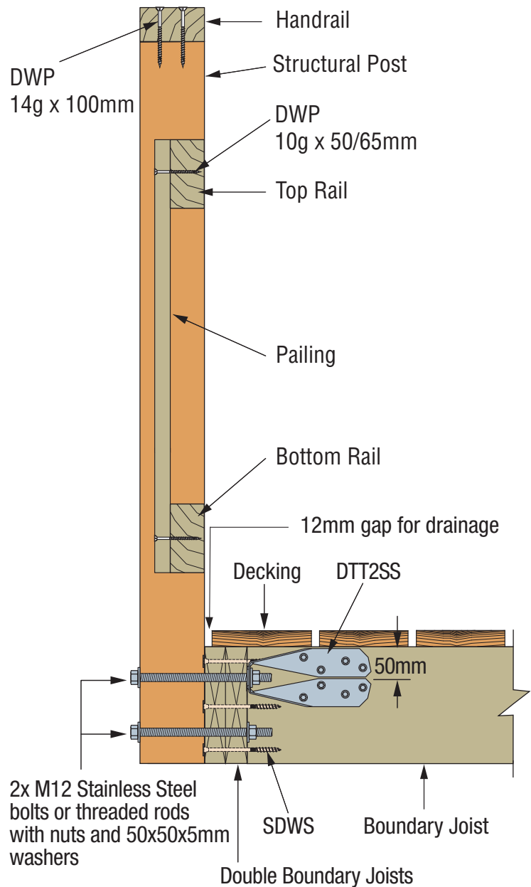
SIMPSON Strong-Tie® SDWS for Cantilever Balustrade with DTT2SS
