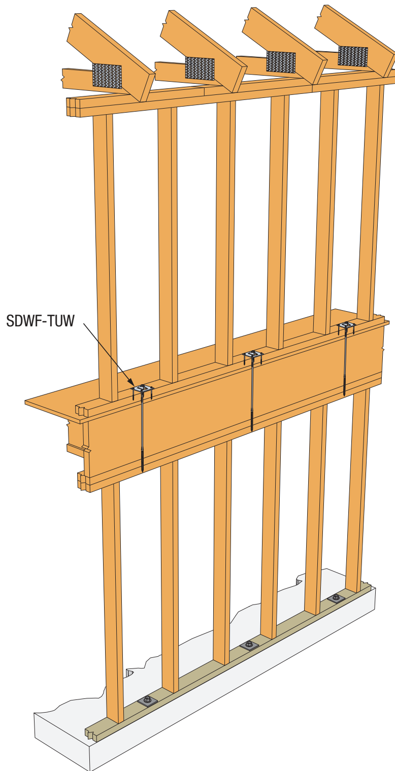
SIMPSON Strong-Tie® SDWF Screw with TUW Take-Up Washer Installation
