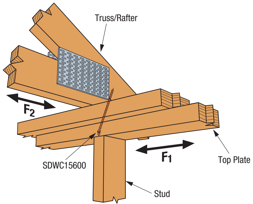
SIMPSON Strong-Tie® SDWC Truss/Rafter-to-Top Plate Installation (Truss aligned with stud)
