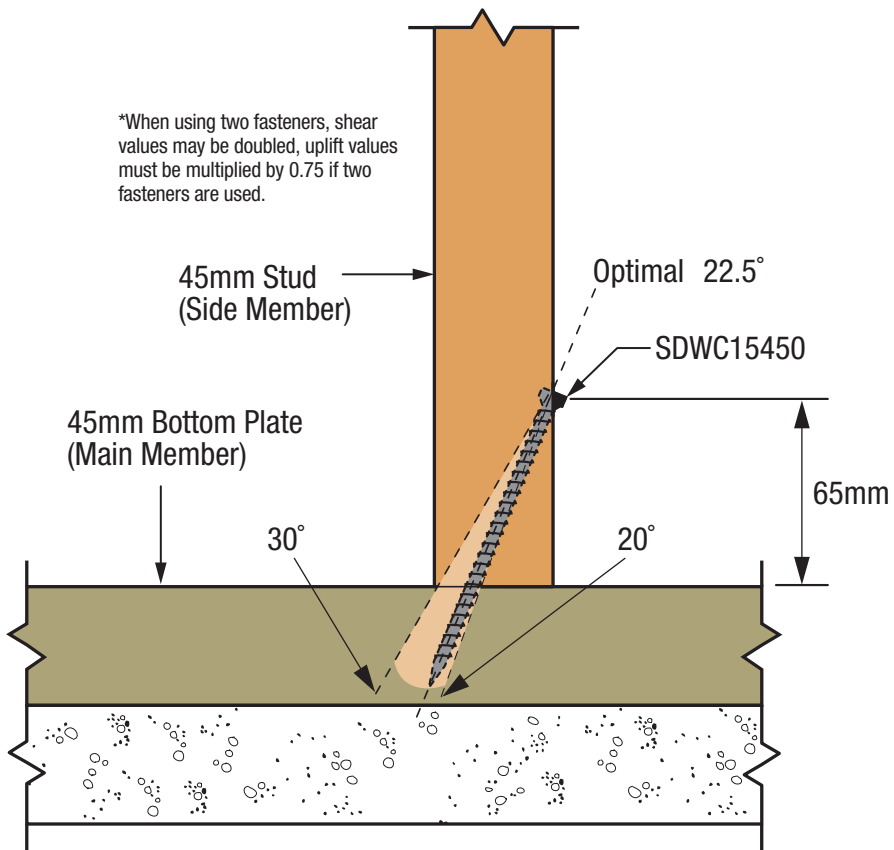
SIMPSON Strong-Tie® SDWC Stud-to-Bottom Plate Installation - Cross Section
