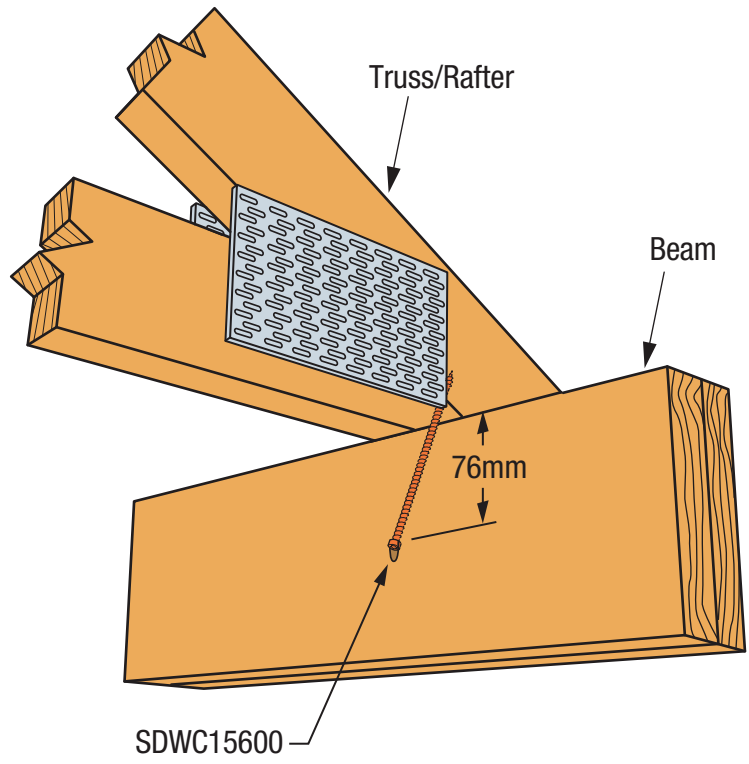
SIMPSON Strong-Tie® SDWC Beam-to-Truss Installation
