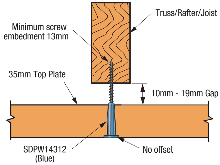
SIMPSON Strong-Tie® SDPW Wall Plate-to-Truss/Joist Installation - Cross Section
