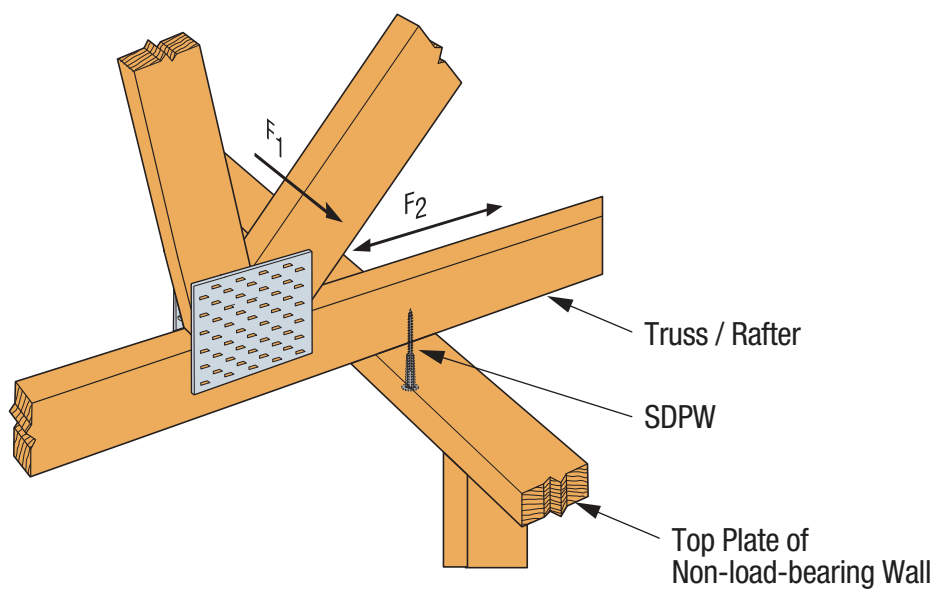
SIMPSON Strong-Tie® SDPW Wall Plate to Truss / Rafter Installation
