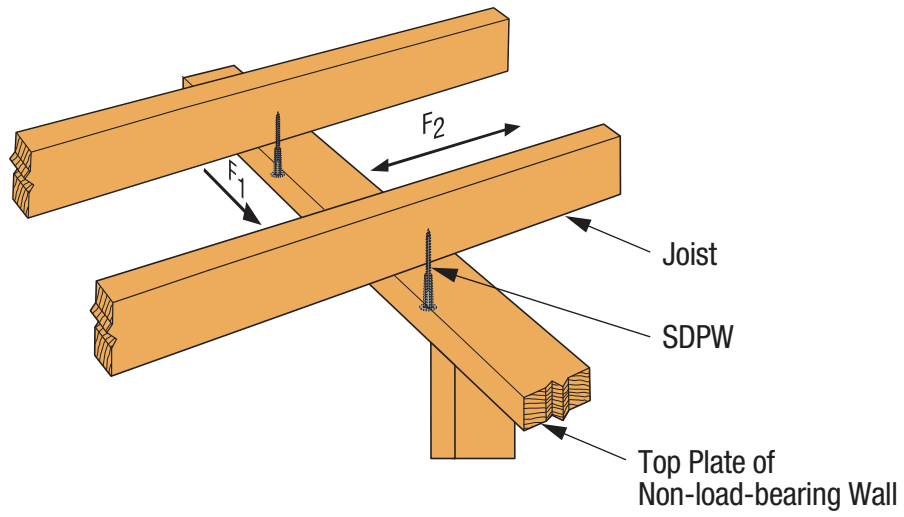
SIMPSON Strong-Tie® SDPW Wall Plate to Joist Installation
