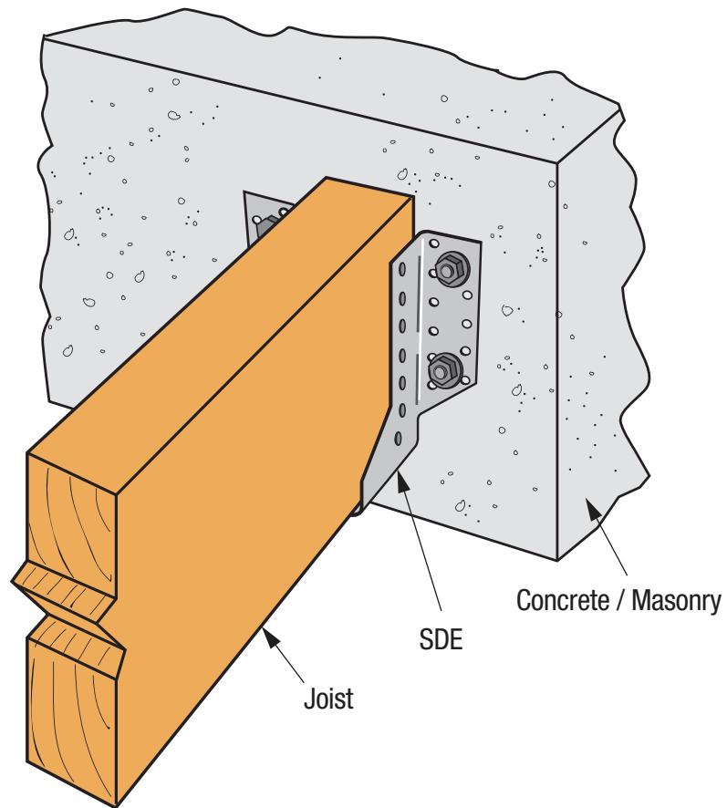
SIMPSON Strong-Tie® SDE Fix Joist on Concrete/Masonry Installation
