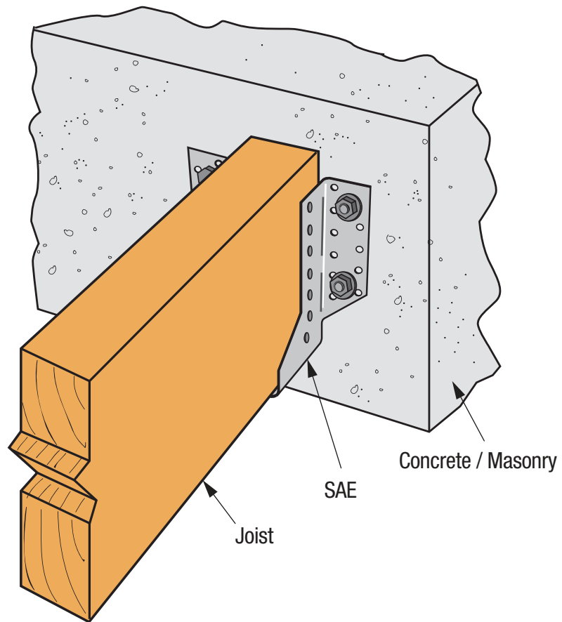
SIMPSON Strong-Tie® SAE Fix Joist on Concrete/Masonry Installation
