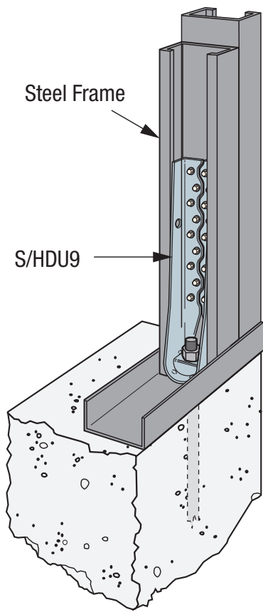
SIMPSON Strong-Tie® S/HDU9 Holddown - Steel Frame
