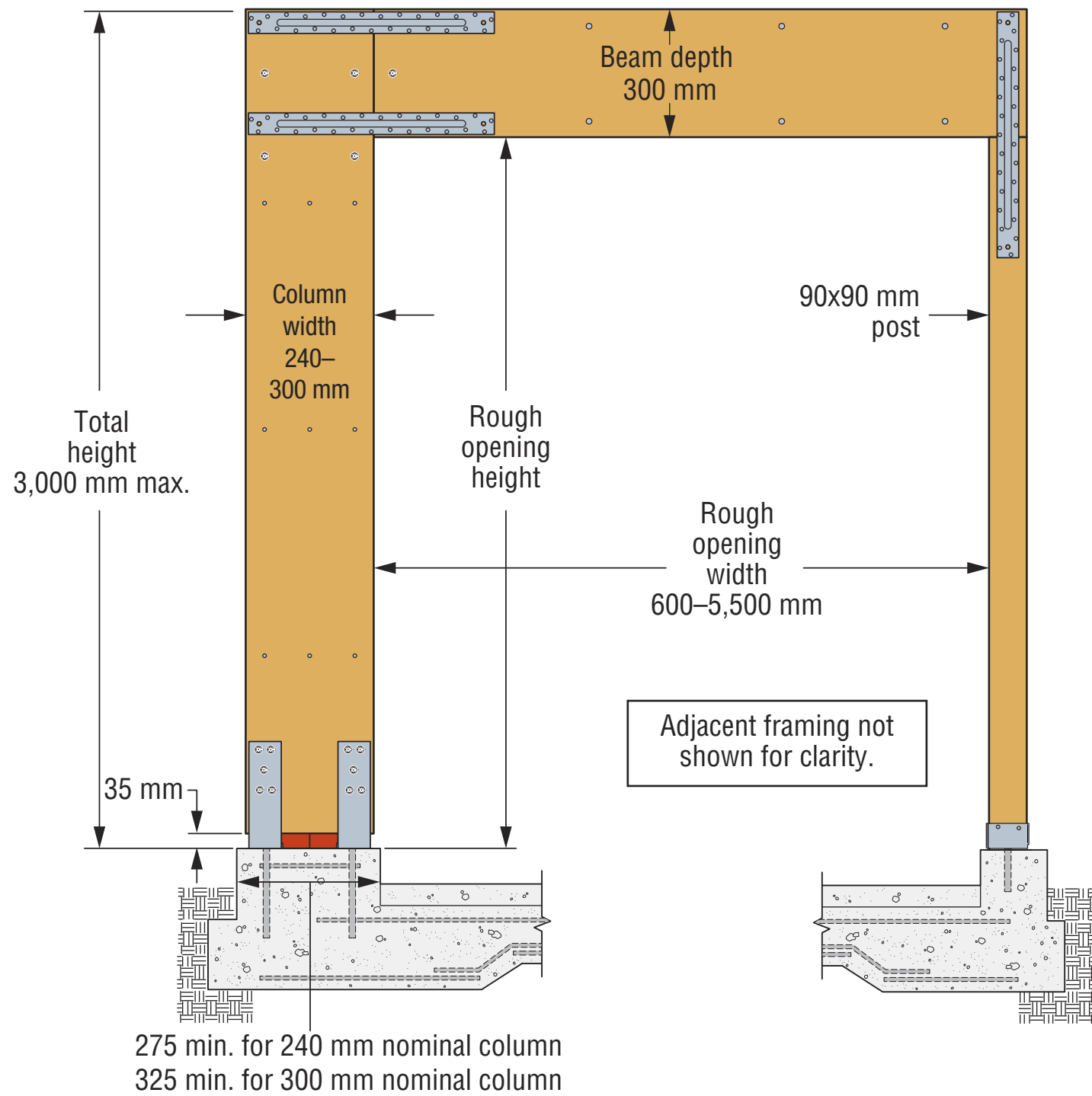
Single-Wall Portal Frame
