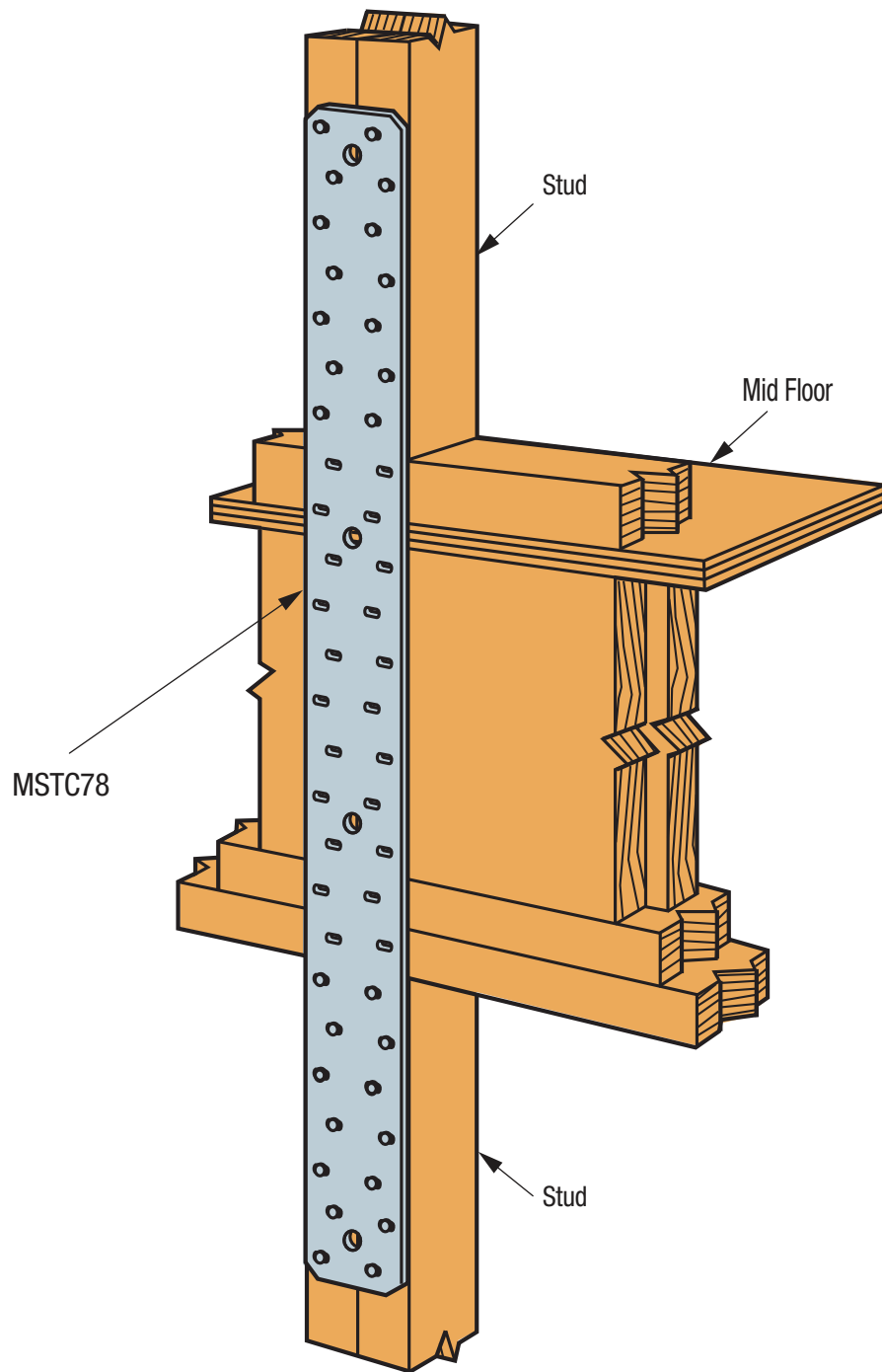
SIMPSON Strong-Tie® MSTC78 Installation
