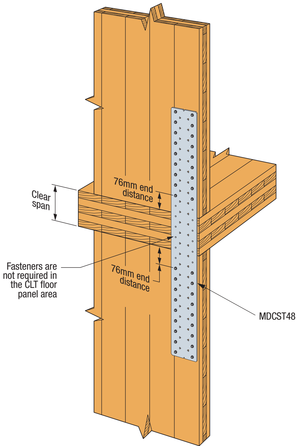
SIMPSON Strong-Tie® MDCST48 Floor-to-Floor Tie Down - CLT Installation
