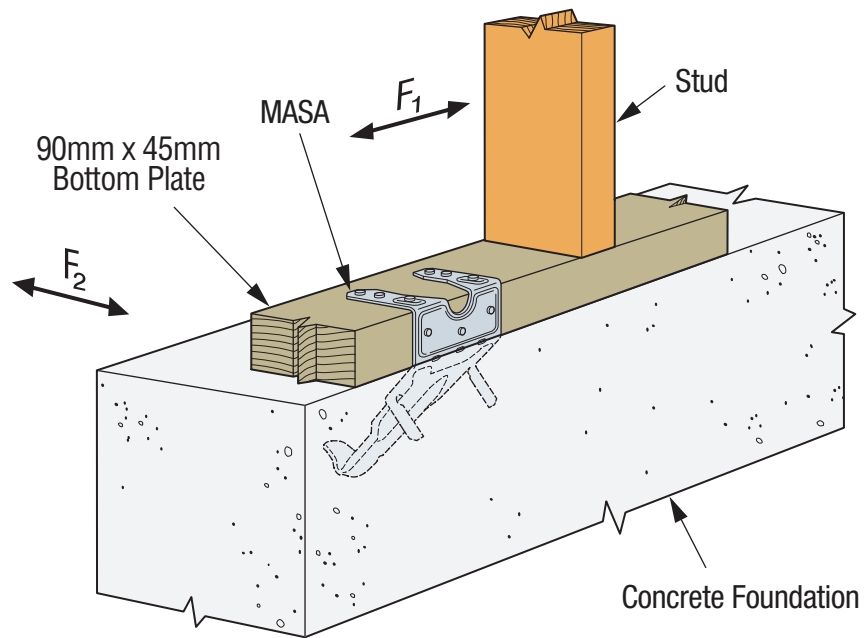
SIMPSON Strong-Tie® MASA Bottom Plate Anchor
