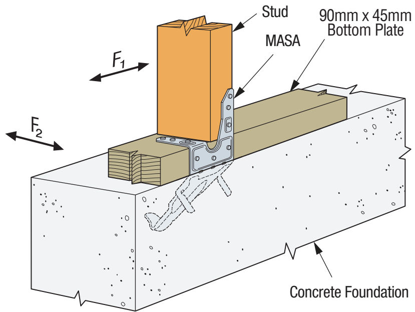
SIMPSON Strong-Tie® MASA Bottom Plate Anchor
