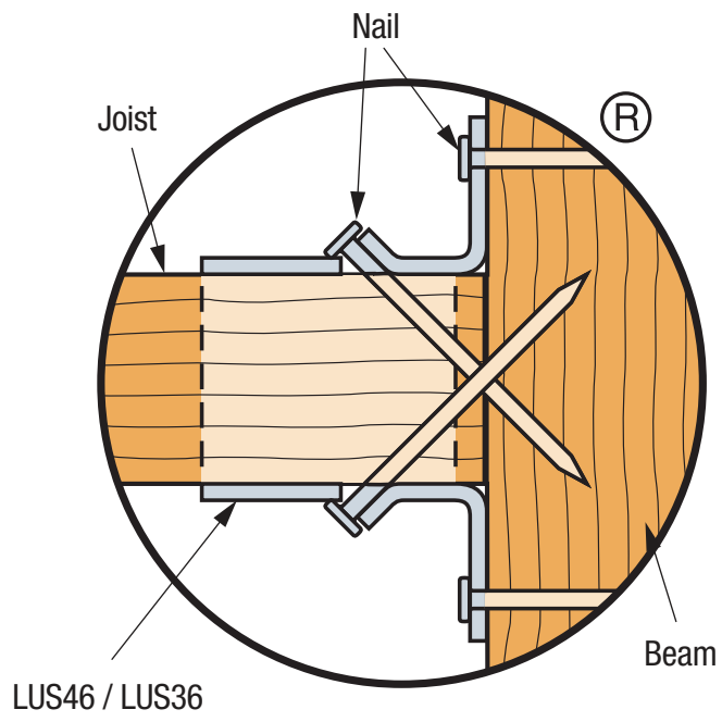
SIMPSON Strong-Tie® LUS46 / LUS36 Double Shear Nailing Installation
