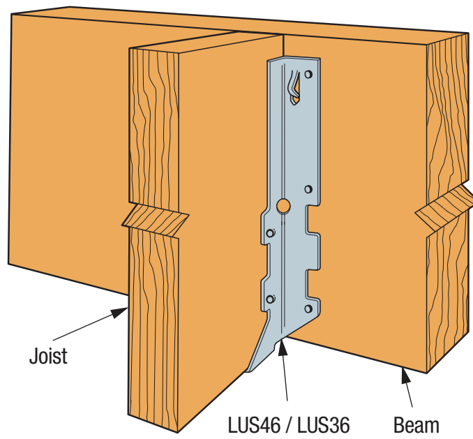
SIMPSON Strong-Tie® LUS Installation
