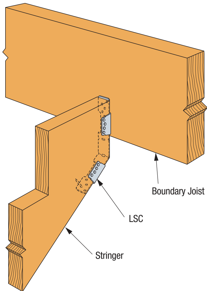
SIMPSON Strong-Tie® LSC Staircase Stringer Connection
