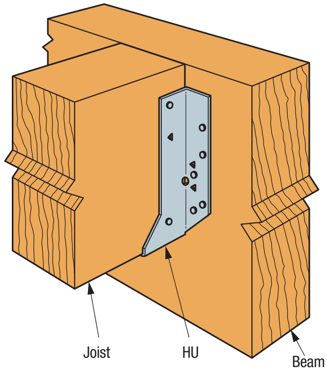
SIMPSON Strong-Tie® HU Face Fix Typical Installation
