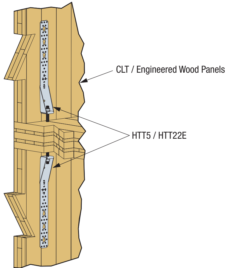
SIMPSON Strong-Tie® HTT Holddown Installation CLT Mid-Floor Connection
