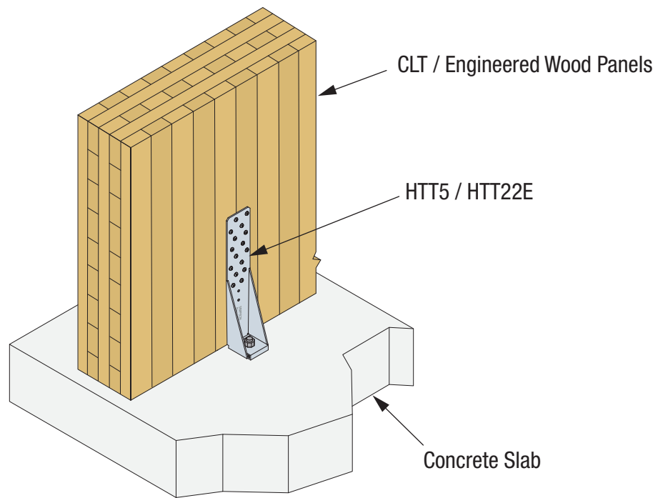
SIMPSON Strong-Tie® HTT Holdown Installation - CLT
