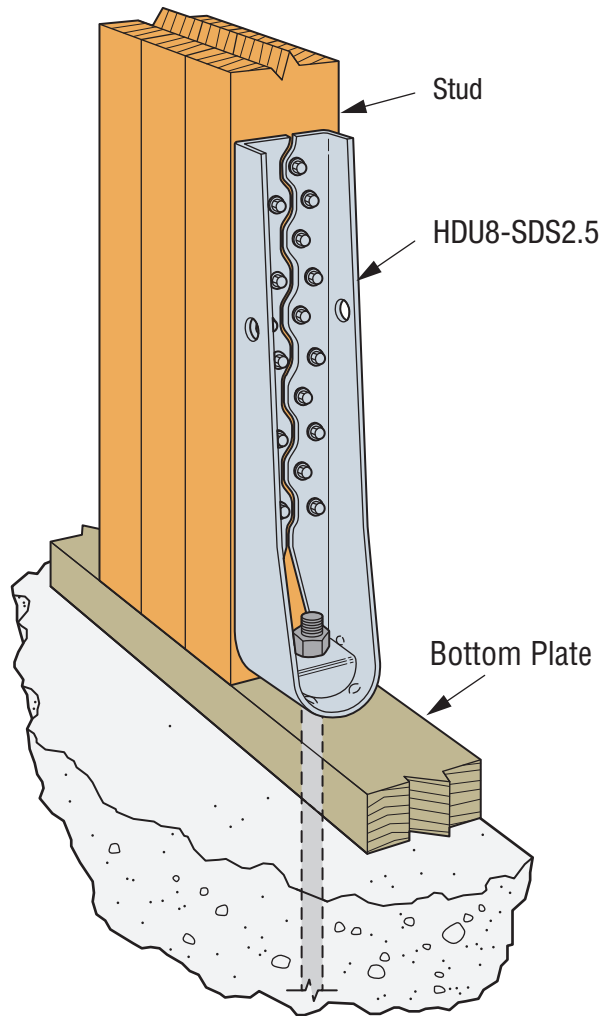
SIMPSON Strong-Tie® HDU8-SDS2.5 Holdown Installation
