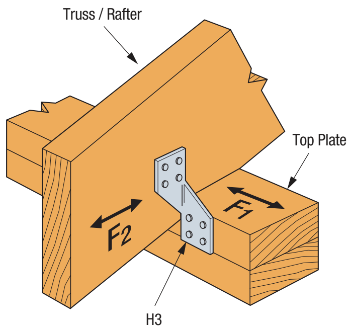
SIMPSON Strong-Tie® H3 Truss/Rafter-to-Top Plate Tie Down
