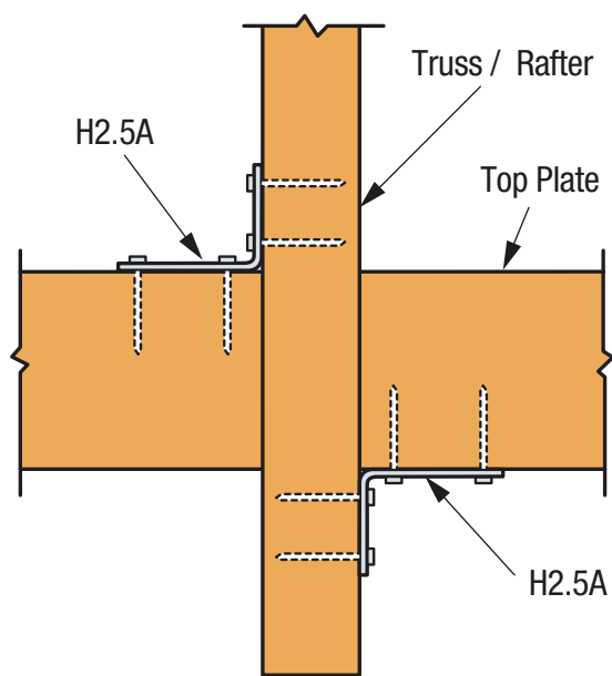
SIMPSON Strong-Tie® H2.5A Truss/Rafter-to-Top Plate Two-Sided Tie Down - Plan View
