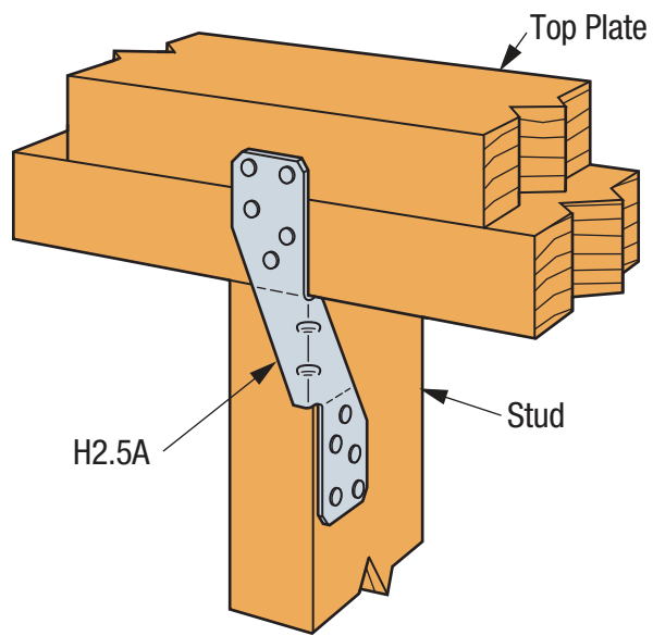
SIMPSON Strong-Tie® H2.5A Stud-to-Top Plate Tie Down
