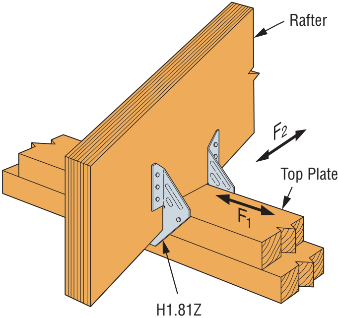
SIMPSON Strong-Tie® H1.81Z Rafter-to-Top Plate Two-Sided Tie Down
