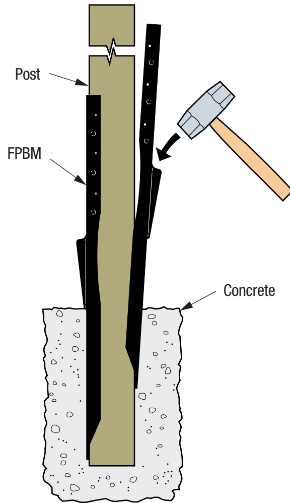
SIMPSON Strong-Tie® E-Z Mender Installation in Concrete
