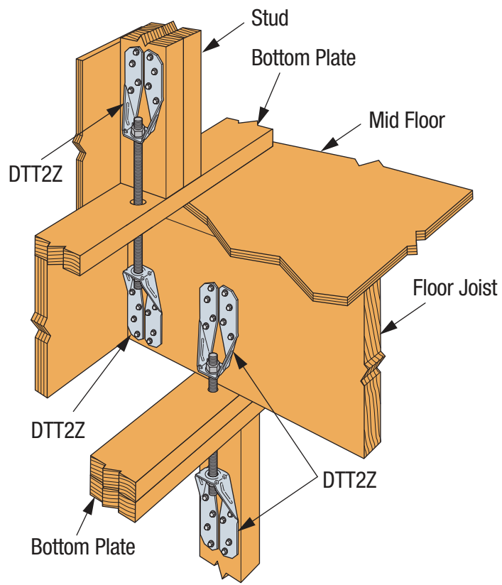
SIMPSON Strong-Tie® DTT2Z Holdown Installation - Vertical Floor
