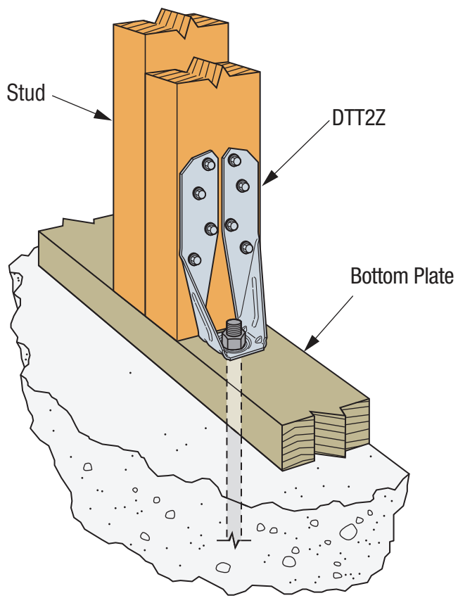
SIMPSON Strong-Tie® DTT2Z Holdown Installation
