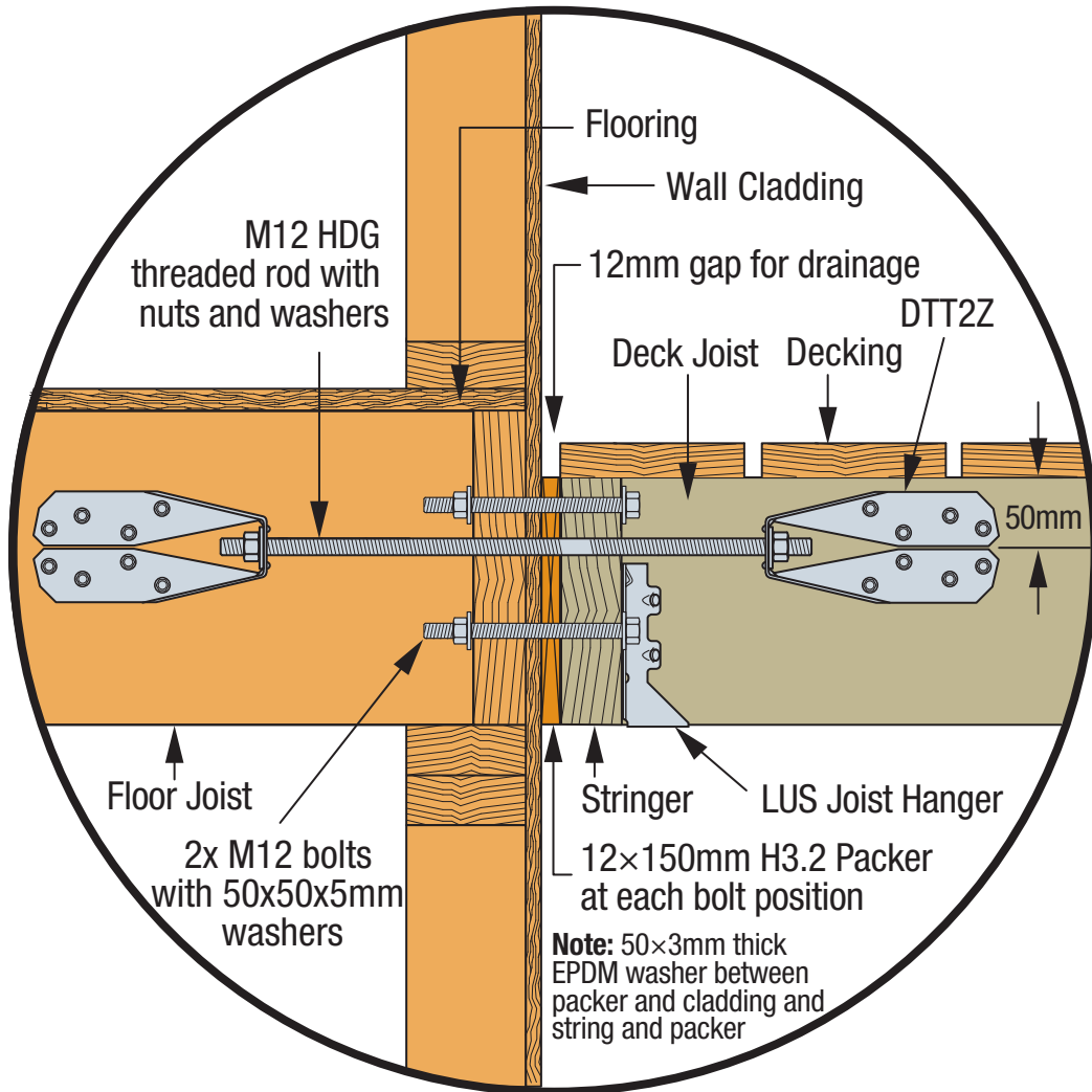
SIMPSON Strong-Tie® DTT2Z Deck-to-House Lateral Load Connection
