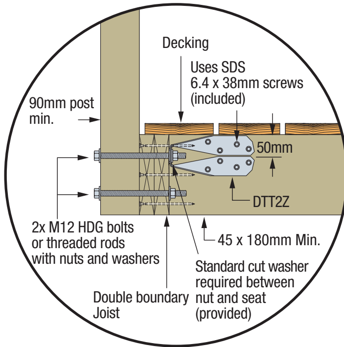
SIMPSON Strong-Tie® DTT2Z Deck Post Connection
