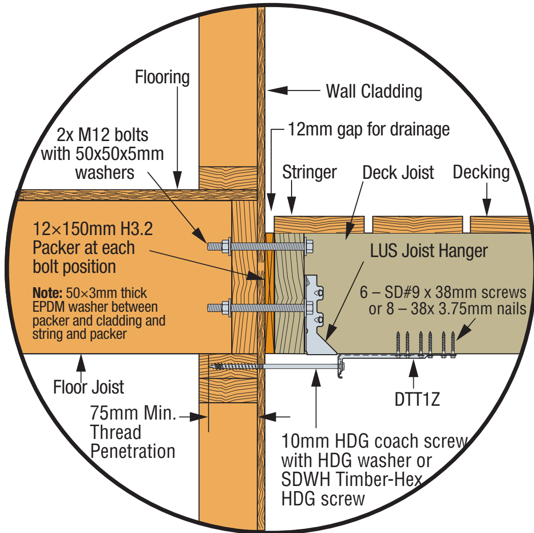
SIMPSON Strong-Tie® DTT1Z Deck-to-House Lateral Load Connection
