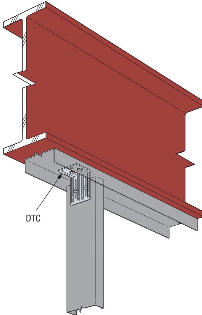
SIMPSON Strong-Tie® DTC Steel Frame Installation
