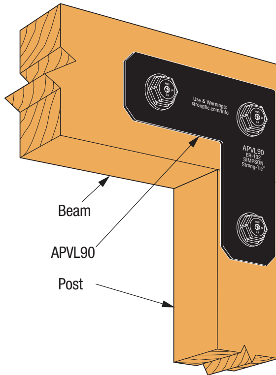
SIMPSON Strong-Tie® APVL90 Post-to-Beam Corner Installation
