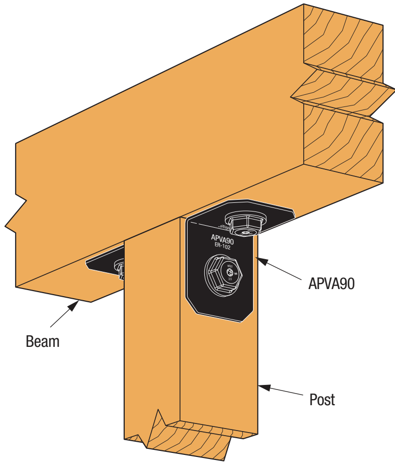
SIMPSON Strong-Tie® APVA Post-to-Beam Installation
