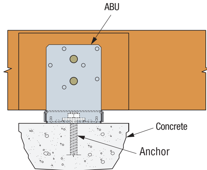
SIMPSON Strong-Tie® ABU Beam Installation
