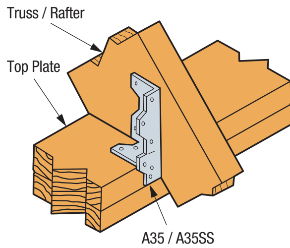
SIMPSON Strong-Tie® A35/A35SS Truss/Rafter-to-Top Plate Installation
